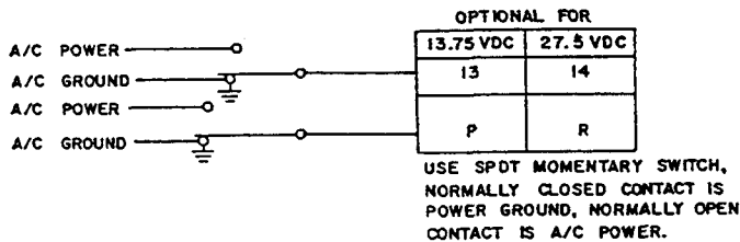
FIGURE 2-5 KX 155 NAV/COMM TRANSCEIVER (Dwg No 155-01343-0000, Rev 3)
