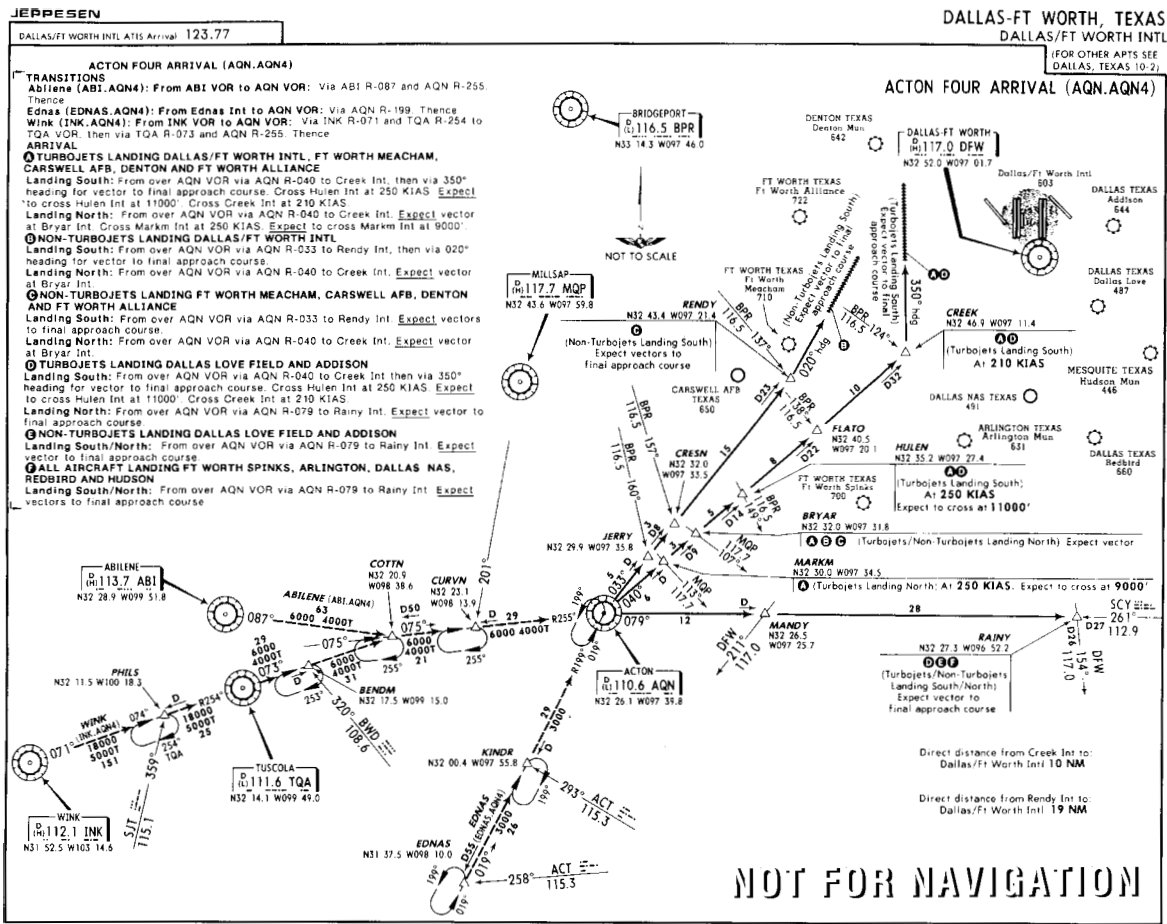
Reproduced with permission of Jeppesen Sanderson, Inc. Reduced for illustrative purposes. Figure 6-44
