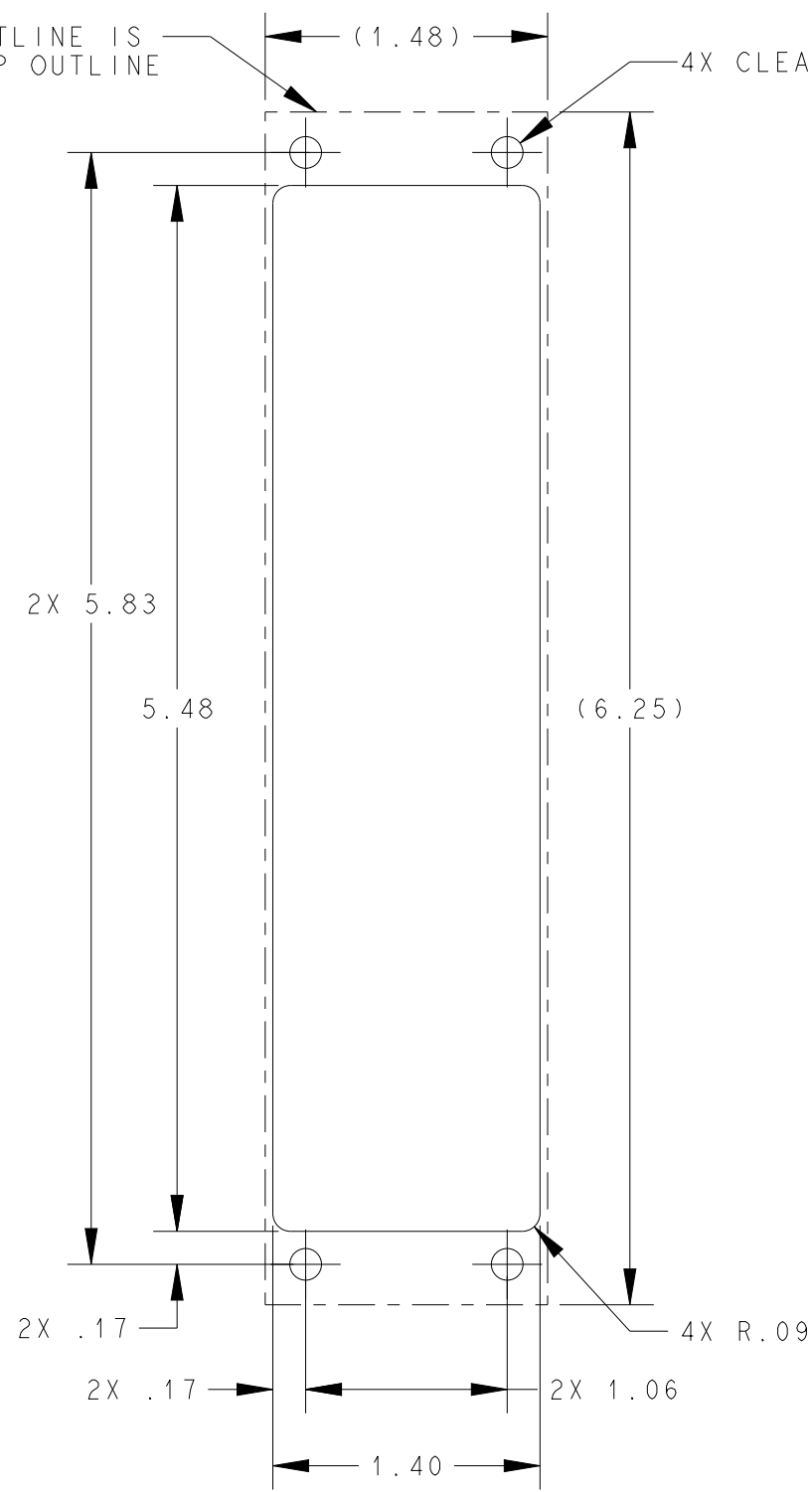
KCP 100EXP CONTROL PANEL (PORTRAIT) - PANEL CUTOUT
