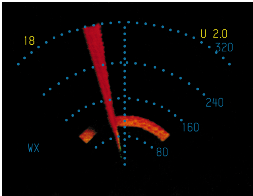
Figure 12: CW Interference
