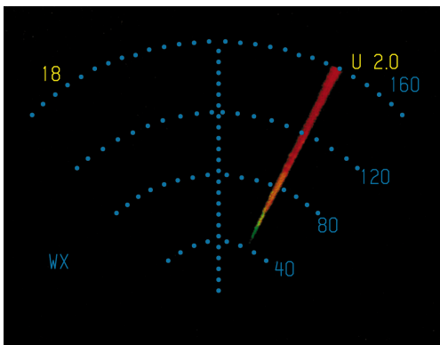
Figure 15: Another Weather Radar's CW Oscillator Interference
