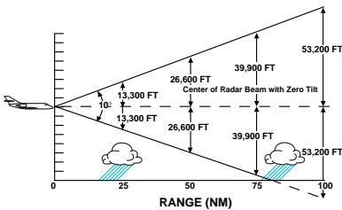
Radar Beam Illumination with 10 Inch Antenna
