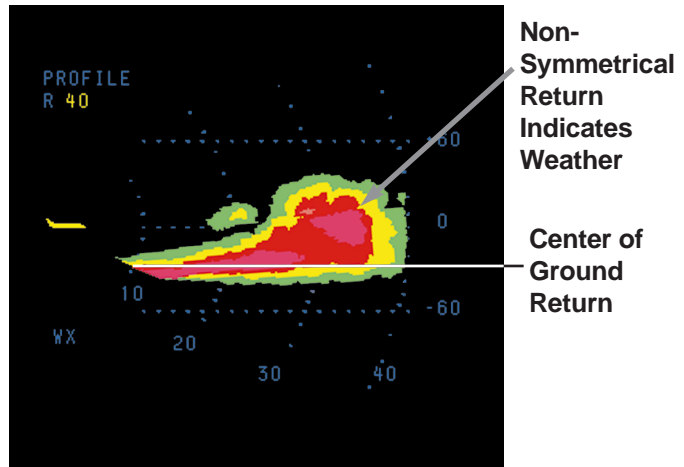
Figure 9: Vertical Profile View Strong Weather Returns Aircraft at 20,000 feet MSL
