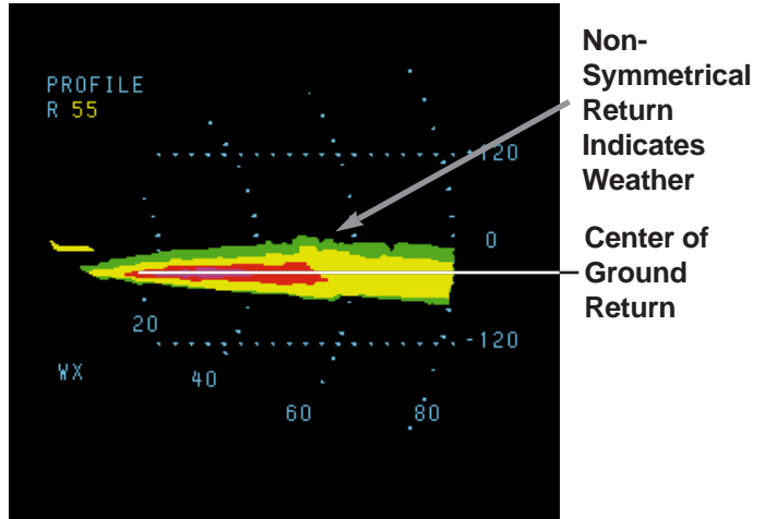
Figure 7: Vertical Profile View Isolated Low Level Weather Aircraft at 20,000 feet MSL
