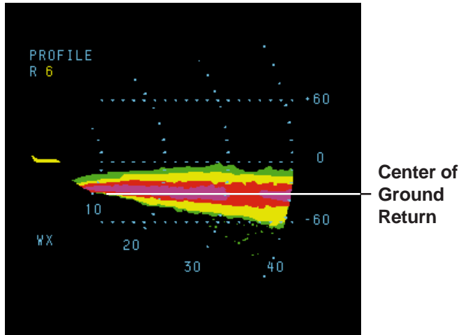
Figure 5: Vertical Profile View Ground Returns Aircraft at 20,000 feet MSL
